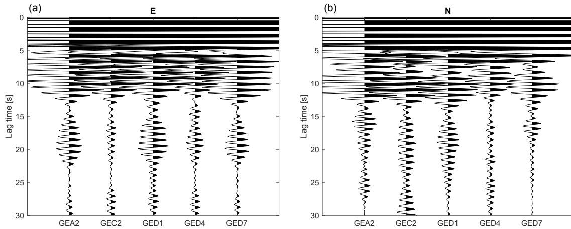
Figure 3.5: Wiggle plots of the calculated horizontal component autocorrelations for the three component stations of the GERESS array. (a) East-West component, (b) North-South component.
