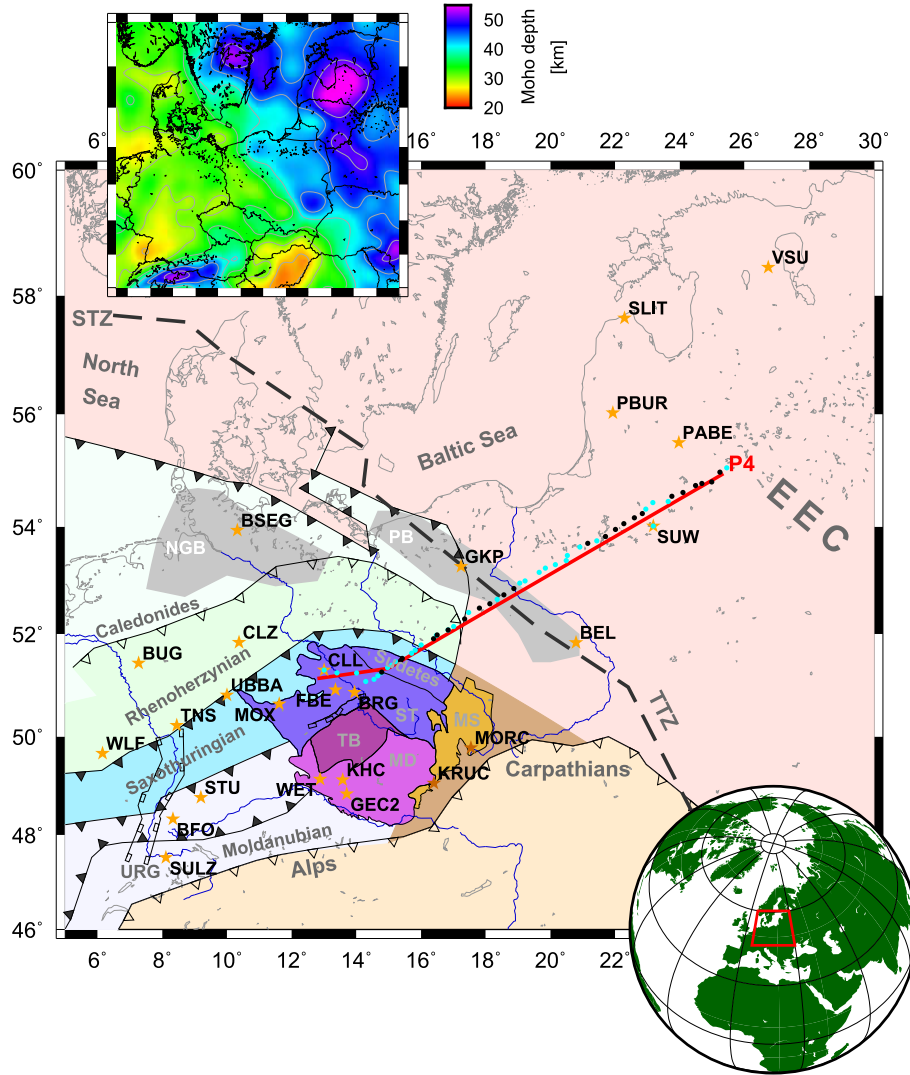
Figure 2.1: Simplified overview of tectonic setting in central Europe (modified after Knapmeyer-Endrun et al. (2014)), along with the stations used. Upper inset shows the Moho map created by Grad et al. (2009). Lower inset: Location of study area. Orange stars: broad-band stations used. Cyan dots: PASSEQ stations used. Black dots: PASSEQ stations along profile P4 not included. Labels: EEC, East European Craton; MD, Moldanubian of Bohemian Massif; MS, Moravo-Silesian of Bohemian Massif; NGB, North German Basin; PB, Polish Basin. ST, Saxothuringian of Bohemian Massif; STZ, Sorgenfrei-Tornquist Zone; TB, Tepla-Barrandian of Bohemian Massif; TTZ, Teisseyre-Tornquist-Zone; URG, Upper Rhine Graben
