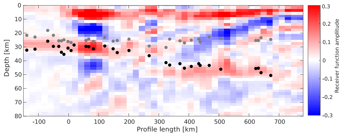
Figure 2.13: Comparison of receiver function result obtained by Knapmeyer-Endrun et al. (2014) with Moho and crustal layer picks, obtained in this study (grey dots: crustal layer; black dots: Moho).
