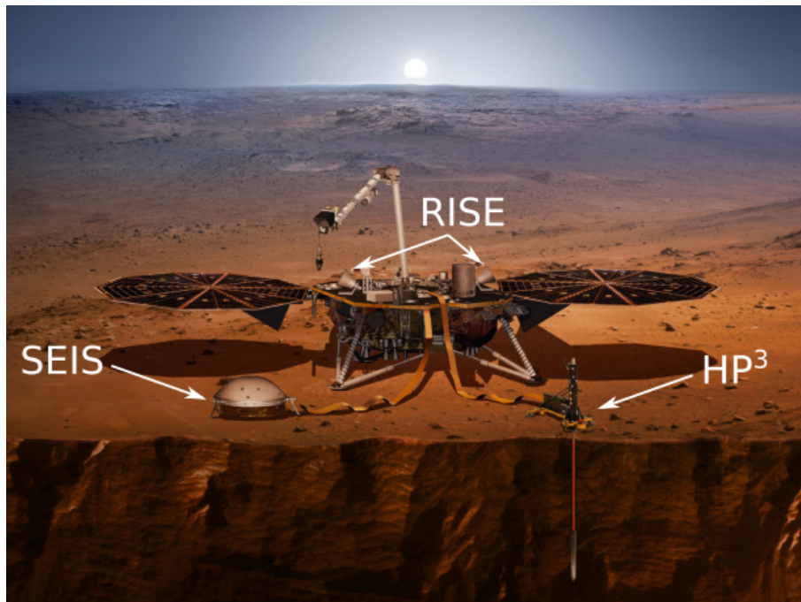
Figure 1.5: Artists view of the InSight lander on Mars, showing the SEIS experiment on the ground on the left and HP 3 on the right. RISE is located on top of the lander. Courtesy of NASA/JPL-Caltech.
