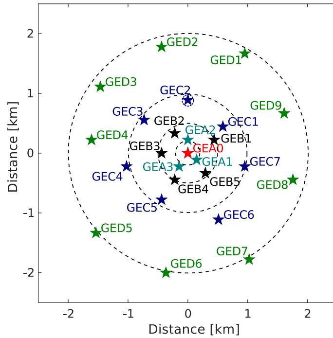
Figure A2.15: Layout of GERESS array. Central point at station GEA0. Stations with the same colours belong to the same ring. Collocated broad-band and short-period station GEC2 is indicated by a circle.
