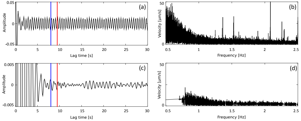
Figure 2.2: Example of spectral smoothing. (a) and (c) show tf-PWS stacked autocorrelation result, filtered between 1 and 2 Hz, for station TNS without and with spectral smoothing. (b) shows a frequency spectrum for an example 3 hr time window of data after high pass filtering and subtraction of the mean and trend. (d) shows the frequency spectrum for the same time window after additional spectral smoothing. Red and blue lines indicate calculated lag time of Moho reflected P -waves according to Grad et al. (2009) and Knapmeyer-Endrun et al. (2014), respectively.
