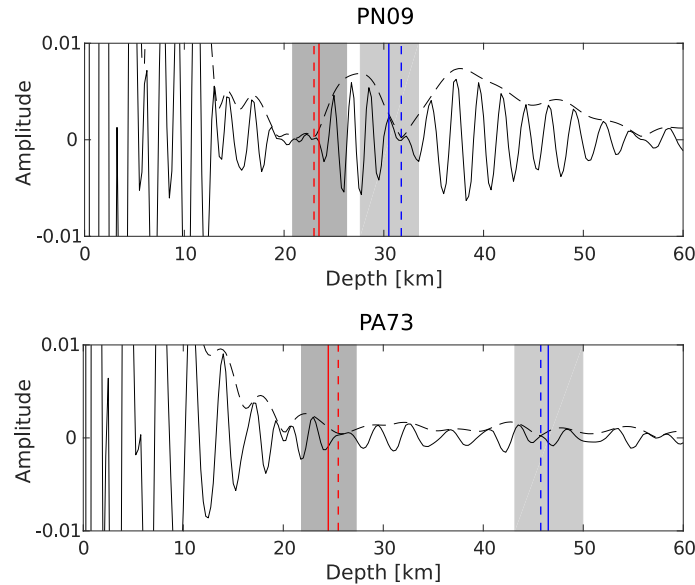
Figure 2.12: Example of intracrustal layer and Moho for stations PN09 and PA73 located at ca. -100 km and 620 km profile length of profile P4 respectively, filtered between 1 and 2 Hz. In red picked (dashed) and given (solid) intracrustal interface. Blue picked (dashed) and given (solid) Moho depth, as seen in profile P4. Picked values correspond to red and blue symbols in Fig. 2.11. Grey areas show 2 km depth and 3 % velocity uncertainty range.
