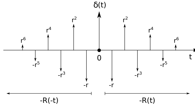
Figure 1.9: Sketch of the autocorrelation T(t) * T(-t) illustrating the associated reflection response R(t) . Modified after Wapenaar et al. (2010).
