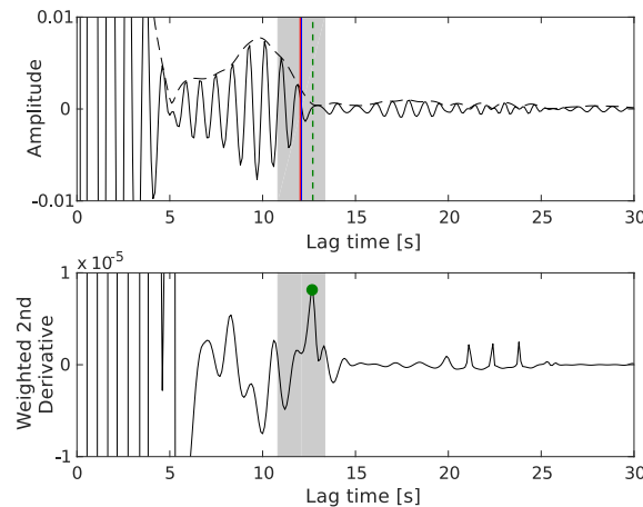
Figure 2.5: Upper image shows stacked and filtered (1-2 Hz) autocorrelation result for station GEC2 with the envelope in dashed black and the highest maximum of the weighted second derivative (bottom panel) in dashed green. The time window, expected to contain the Moho reflection, based on prior information, is marked in grey. Red and blue lines (overlapping) indicate calculated lag time of Moho reflected P -waves according to Grad et al. (2009) and Knapmeyer-Endrun et al. (2014).
