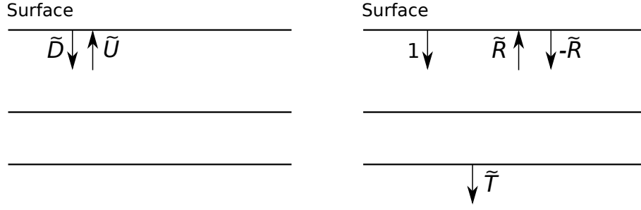
Figure 1.10: Sketch of a layered medium indicating in the frequency domain the down-going plane wave-field \tilde{D} , the up-going plane wave-field \tilde{U} on the left and a plane wave travelling down 1, the up- and down-going reflection responses \tilde{R} and -\tilde{R} and the total down-going transmitted wave-field \tilde{T} on the right.
