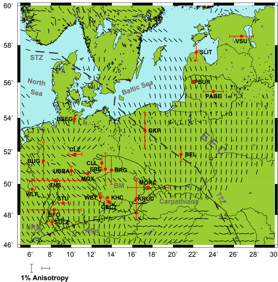
Figure 3.11: Overview of determined anisotropy orientation and value over-plotted onto the smoothed world stress map by Heidbach et al. (2010). The red lines are oriented in direction of the component registering earlier arrival, with the lengths proportional to percentage of anisotropy. For labels refer to Fig. 3.1.
