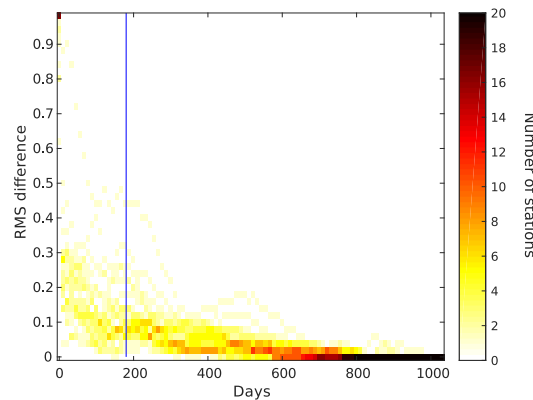
Figure 2.8: Data-density plot of the normalized RMS-value of difference between final stack result and continuous stacking of autocorrelations for different broad-band stations. Blue line indicates the 180 day cut-off.
