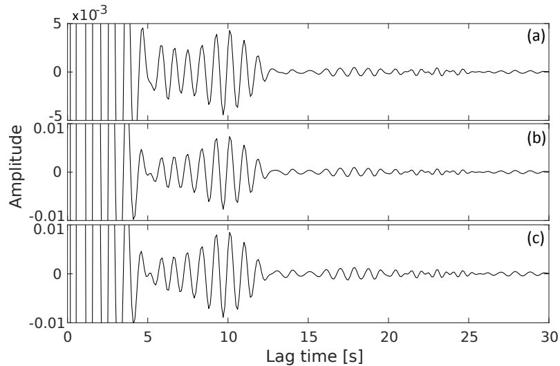
Figure A2.17: Comparison of stacked autocorrelation results for broad-band station GEC2 with window length of 1 hr (a), 3 hr (b) and 6 hr (c) used for the calculation of the autocorrelations. The number of stacked windows is: 22747 windows for 1 hr length (= 948 d), 5571 windows for 3 hr length (= 696 d) and 1762 windows for 6 hr length (= 440 d).
