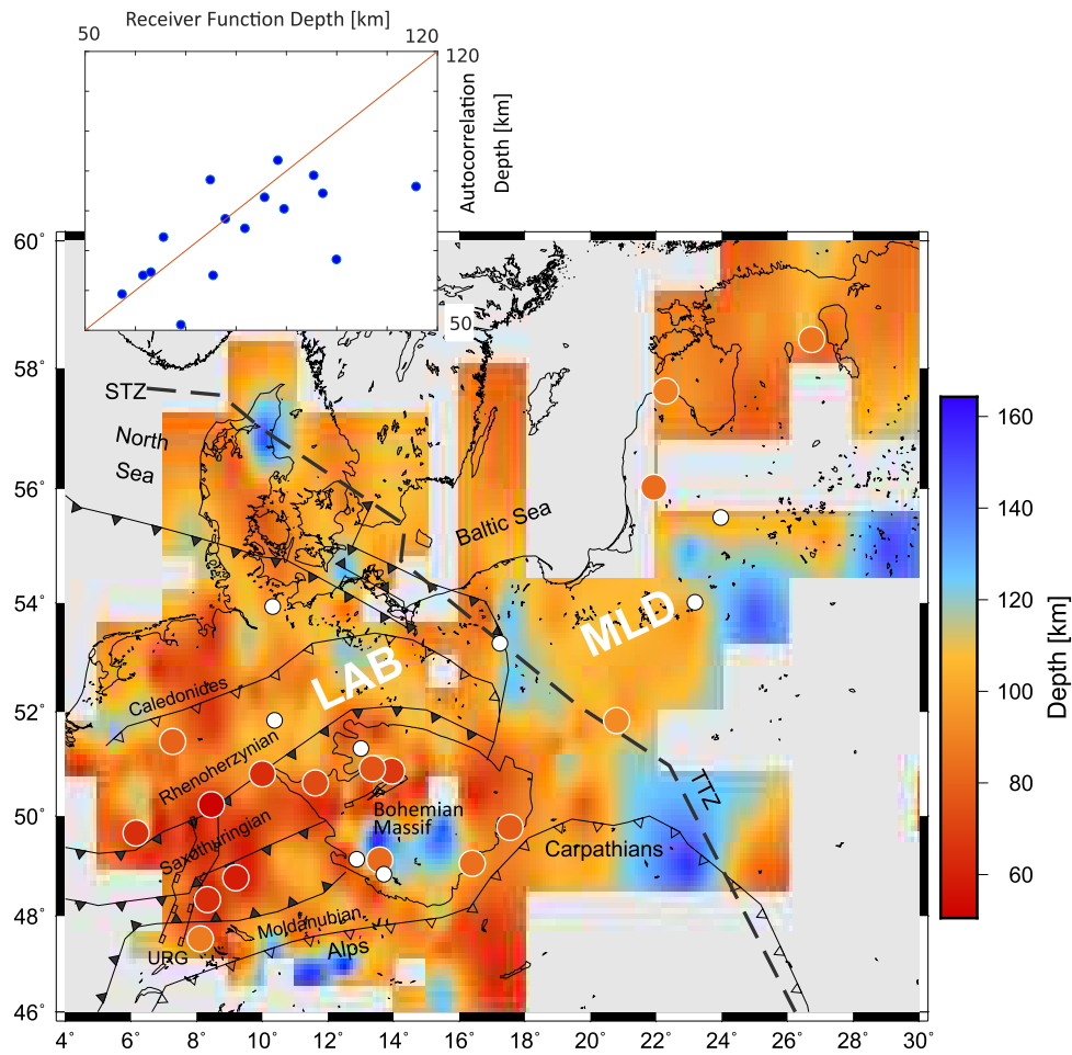
Figure 2.14: Map of lithosphere-asthenosphere boundary depth west of the TESZ and mid-lithosphere depth east of the TESZ from Knapmeyer-Endrun et al. (2017b). The broad-band station locations and determined depths, based on autocorrelations filtered between 1-2 Hz, are indicated by circles. White circles indicate stations without later increase in autocorrelation amplitude. The inset on top shows the depth obtained by receiver functions versus the depth determined from the autocorrelations. The red line has a slope of one. For labels refer to Fig. 2.1.
