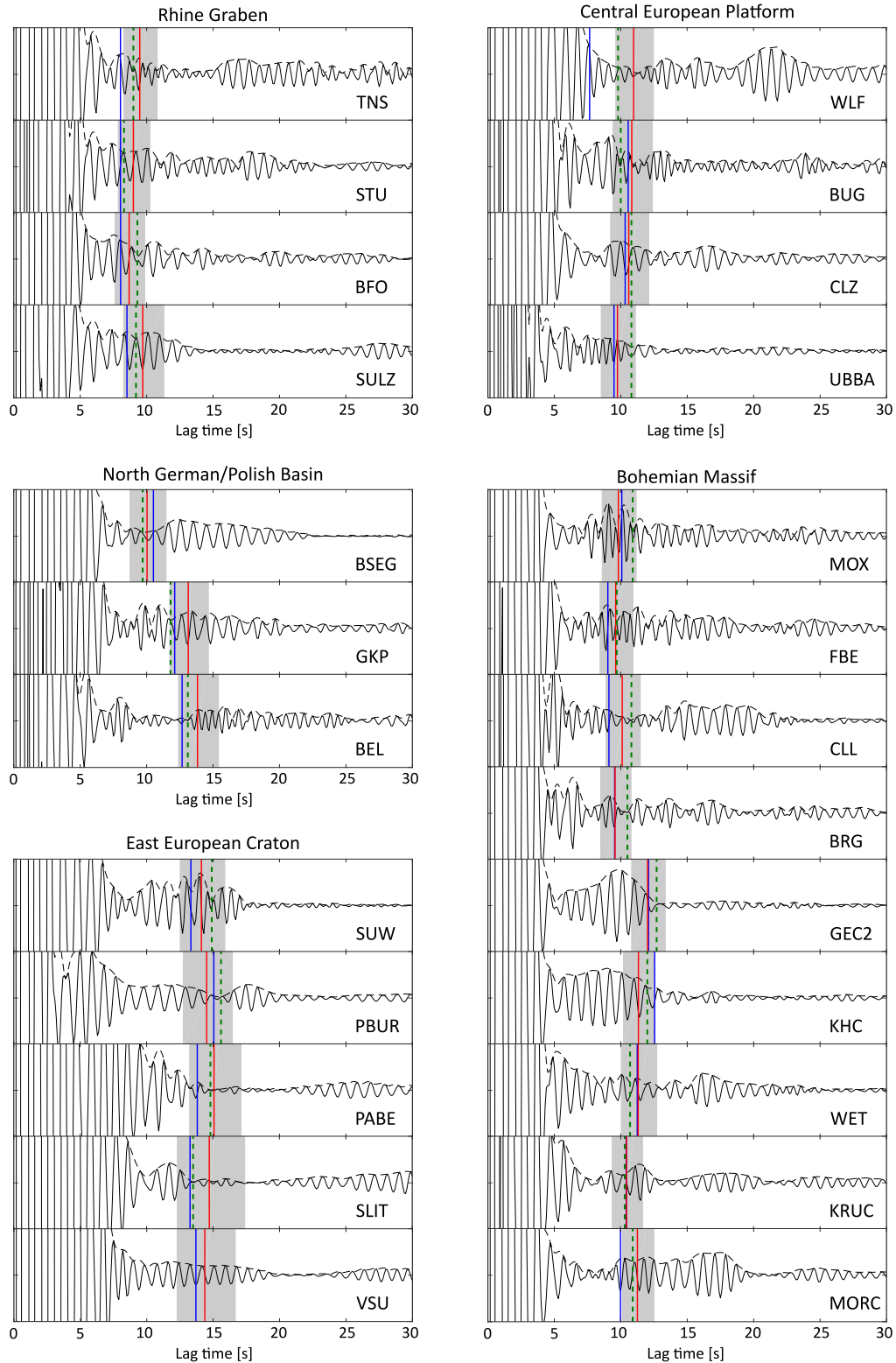
Figure 2.9: Autocorrelations, filtered between 1 and 2 Hz, in black with envelopes (dashed, black) and results of automatically picked arrival times of Moho reflections (dashed, green), along with calculated times obtained from Knapmeyer-Endrun et al. (2014) (blue) and Grad et al. (2009) (red). Grey area indicates 5 % velocity uncertainty combined with depth uncertainty provided by Grad et al. (2009).
