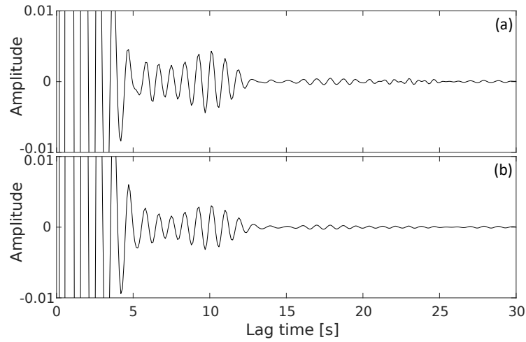
Figure A2.16: Comparison of tf-PWS stacked autocorrelation result for broad-band station GEC2 for window length of 1 hr, without removal of the instrument response in (a). (b): same processing as in (a), but a restitution filter to remove the instrument response is included before any other processing steps.
