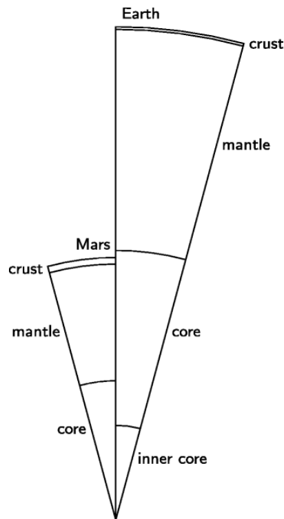
Figure 1.2: Sketch of the internal structure of Mars with respect to Earth (taken from Helffrich (2017)).
