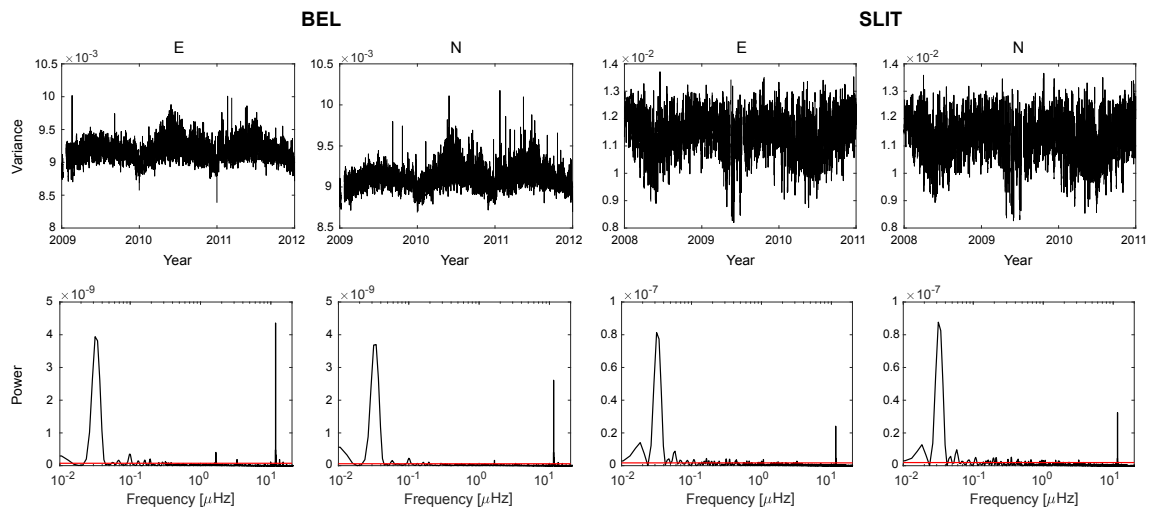
Figure 3.3: Temporal properties of autocorrelations from stations BEL and SLIT for the two horizontal components. Top row: Calculated variances for 0-30 s lag time. Bottom row: Corresponding Lomb-Scargle-Periodograms. Red line: 99 % threshold of the frequency peak being a random fluctuation.
