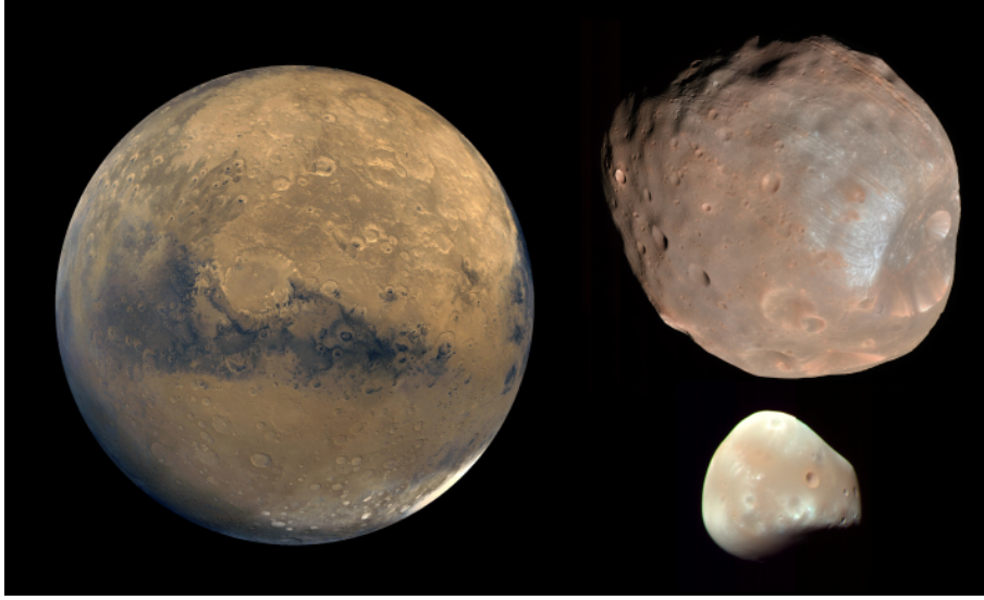
Figure 1.1: Left: Mosaic image of Mars composed of 100 Viking Orbiter images taken in 1980. Right: HiRISE images taken from Mars Reconnaissance Orbiter Phobos (top) and Deimos (bottom). Images not to scale. Courtesy of NASA/JPL-Caltech/USGS/University of Arizona.
