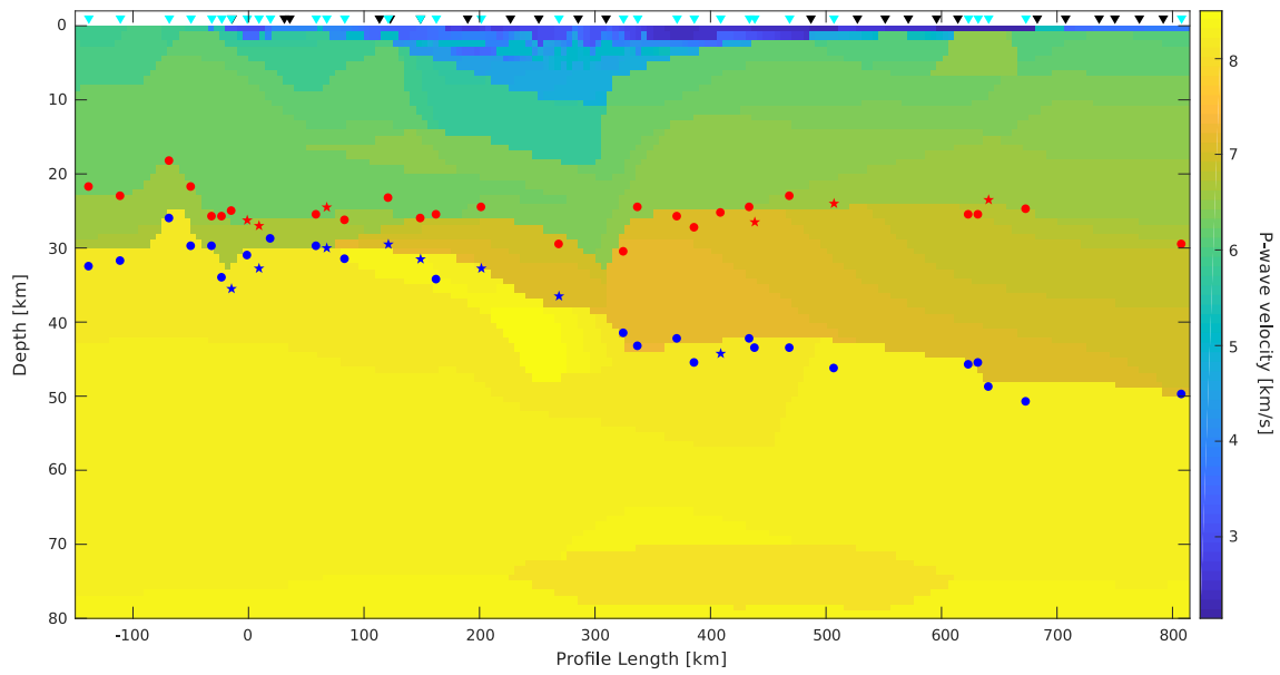
Figure 2.11: Changes in reflectivity derived from autocorrelation of PASSEQ stations along POLONAISE P4 profile from west to east, with the velocity model by Grad et al. (2003) used to convert lag time to depth in the background. Cyan inverted triangles: stations used; black inverted triangles: stations discarded due to faulty or too little data; blue dots: picked changes in reflectivity at Moho depth in the 1-2 Hz frequency band; blue stars: picked changes in reflectivity at Moho depth in 2-4 Hz frequency band; red dots: picked changes in reflectivity at intracrustal interface in 1-2 Hz frequency band; red stars: picked changes in reflectivity at intracrustal interface in 2-4 Hz frequency band.
