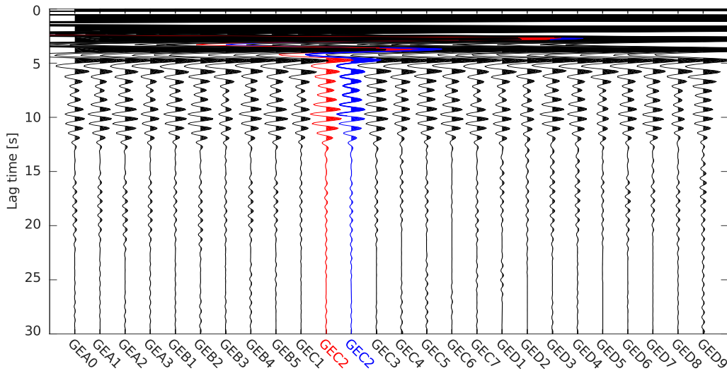
Figure 2.6: Comparison of autocorrelation results for the stations of the GERESS array, filtered between 1 and 2 Hz. Red and blue traces depict the comparison of collocated broad-band and short-period seismometer, respectively.
