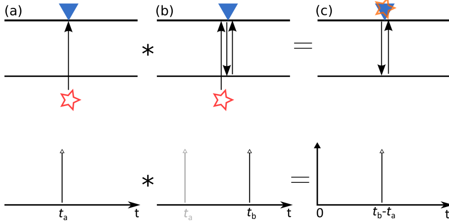
Figure 1.8: Sketch of the theory of seismic interferometry. (a): a seismic wave travels from a source at depth (red) to a seismic station (blue) on the surface and is recorded at time t_a . (b): The seismic waves reflected downward at the surface and upward at the interface and recorded at time t_b . (c): The autocorrelation of the signal results in the seismic station and a virtual source (orange) being collocated and seismic wave travelling down and being reflected upward again, reaching the station at time t_b - t_a . Modified after Schuster (2009).
