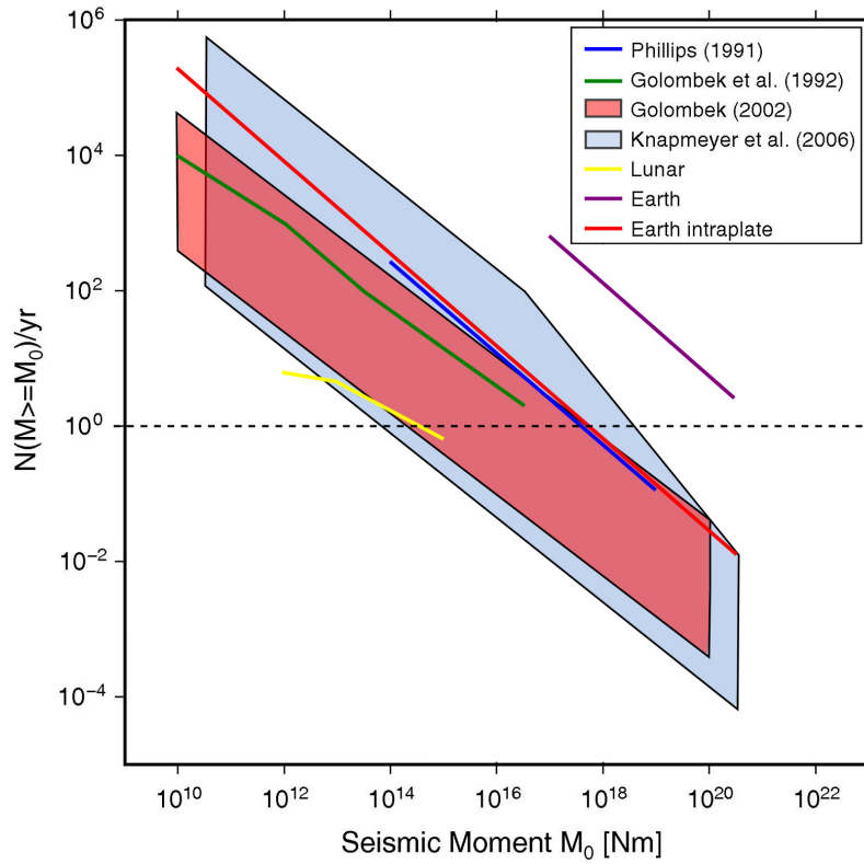
Figure 1.6: Comparison of the estimates of size-frequency distributions of seismic events obtained from different studies, as well as distributions for the Earth and Moon (adapted and compiled from Knapmeyer et al. (2006), Panning et al. (2015)). Dashed horizontal line indicates the level above which events would be expected to be seen during the InSight mission (Panning et al. 2015).
