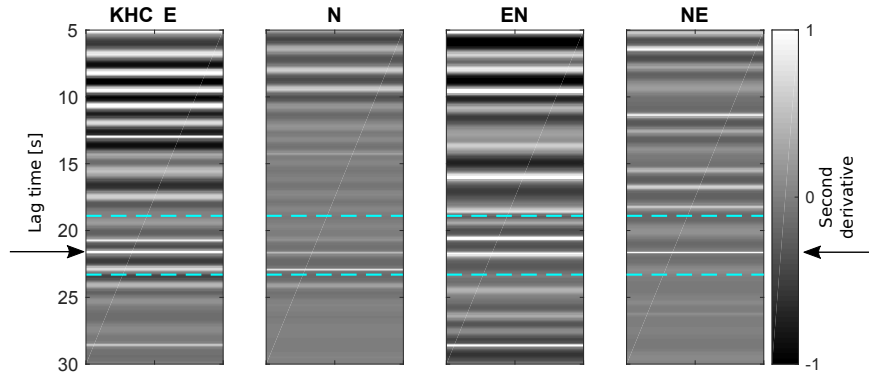
Figure 3.2: Second derivatives of horizontal correlations of station KHC filtered between 1 and 2 Hz. Grey shading of image-plot depends on the amplitude of the second derivative. Cyan lines indicate the calculated target window. Arrows point to reflectivity change visible in all correlations.
