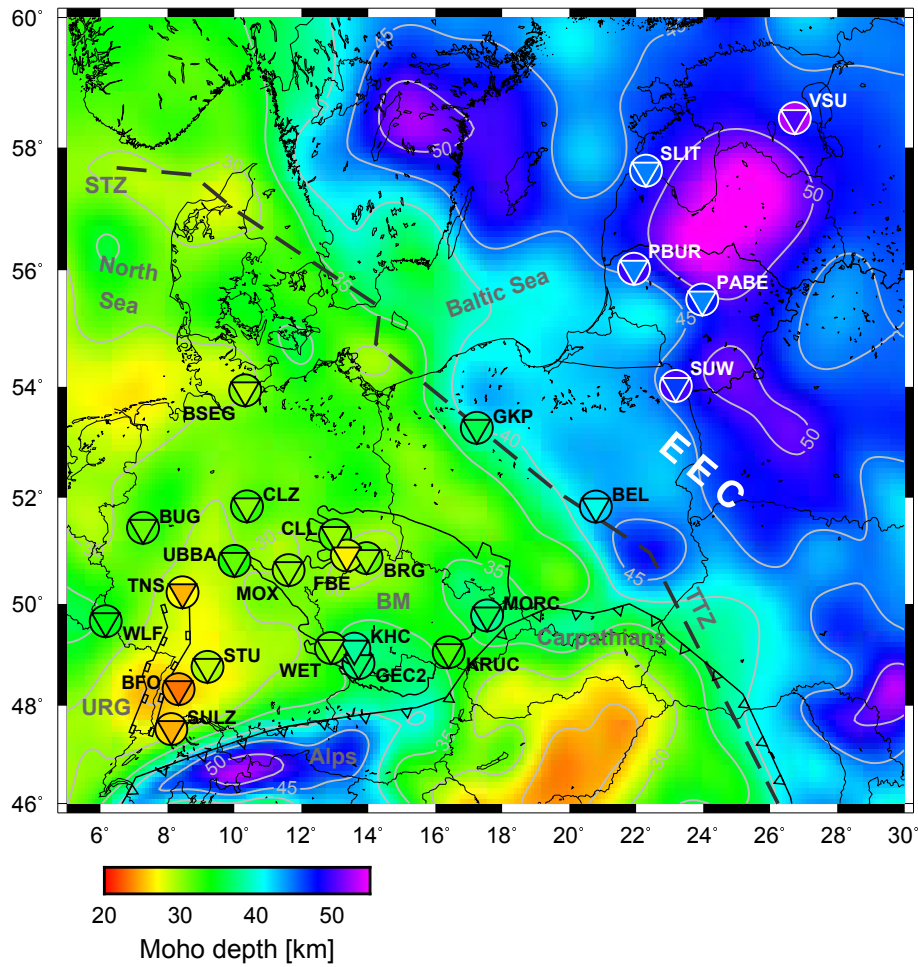
Figure 3.9: Moho depth ranges obtained from auto- and cross-correlations of horizontal components over-plotted on the European Moho depth map after Grad et al. (2009). Circles indicate lower boundary, triangles upper boundary. Labels: BM: Bohemian Massif; EEC: East European Craton; STZ: Sorgenfrei-Tornquist-Zone; TTZ: Teisseyre-Tornquist-Zone; URG: Upper Rhine Graben.
