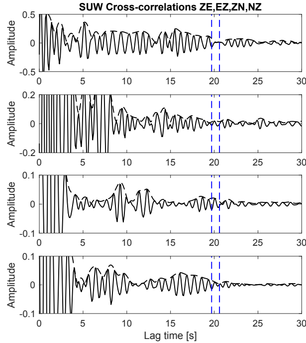
Figure 3.6: Vertical-horizontal components cross-correlations (black) of station SUW. Black dashed line: envelope. Blue lines: Calculated expected lag times from vertical component autocorrelation and horizontal component auto- and cross-correlation picks.
