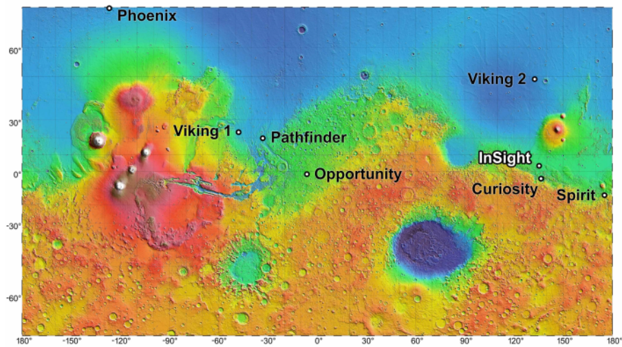
Figure 1.4: Topographic map of Mars constructed from Mars Orbiter Laser Altimeter data, indicating the planned landing site of the InSight mission, along with landing site of former missions. Lowest elevations in dark blue; highest elevations white. Elevation difference between green and orange approximately 4 km. Courtesy of NASA/JPL-Caltech.
