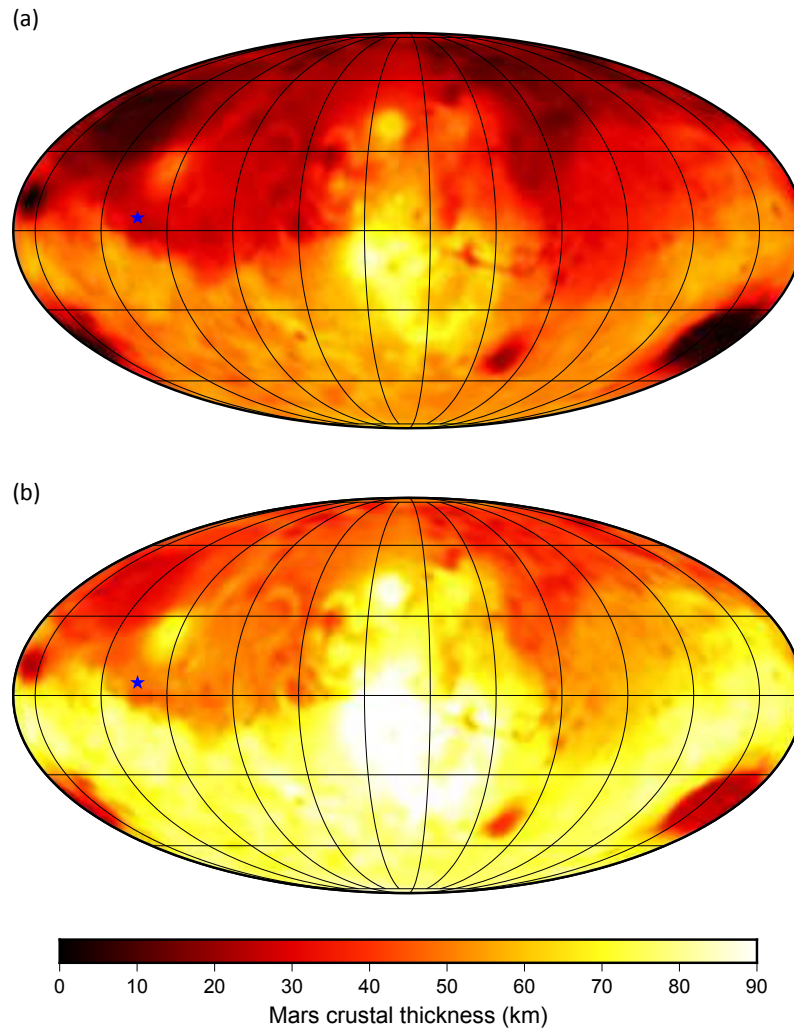
Figure 1.3: Comparison of two Martian crustal thickness estimates for an average crustal density of 2900 \text{ kg m}^{-3} after Plesa et al. (2016). Blue star indicates InSight landing site (Golombek et al. 2017). (a) Minimum crustal thickness of 1 km, resulting in an average crustal thickness of 40 km. (b) Minimum crustal thickness of 20 km, resulting in an average crustal thickness of 63.3 km.
