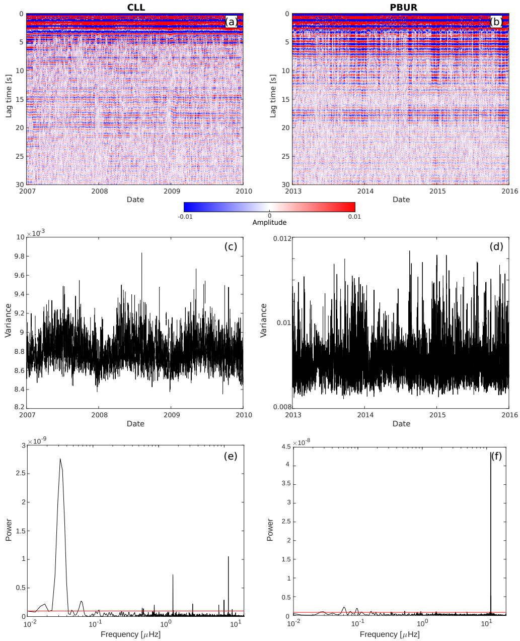
Figure 2.7: Top: Daily stacks of autocorrelations for stations CLL (a) and PBUR (b), filtered between 1 and 2 Hz. (c,d) Variance over time. (e,f) Power spectra calculated with the Lomb-Scargle method from the variances of the single autocorrelations. The red line shows the 99 % probability threshold of not being a random fluctuation.
