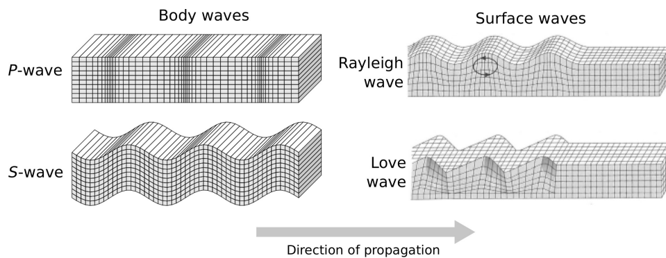
Figure 1.7: Overview of the particle motion for the different seismic wave types. Body waves after Shearer (2009) and surface waves after Fowler (2005).
