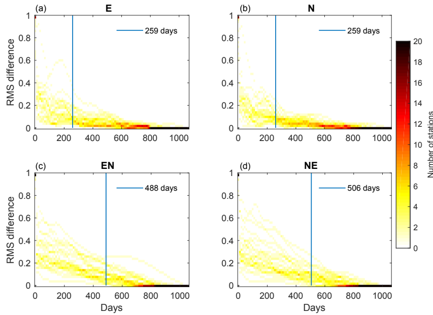
Figure 3.4: Data density plots of the root-mean-square (RMS) difference of the final linear stack with continuously stacked autocorrelations (a,b) and cross-correlations (c,d). Blue lines indicate the threshold, after which the median RMS-difference permanently decreases to below 0.1.
