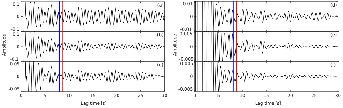
Figure 2.3: Application of different stacking algorithms to autocorrelations for station BFO. All results are filtered between 1-2 Hz. Left: stacking applied to autocorrelations without spectral smoothing; right: autocorrelations calculated with spectral smoothing. (a,d): Linear stack; (b,e): phase-weighted stack according to eq. 2.2 (Schimmel & Paulssen 1997); (c,f): time-frequency domain phase weighted stack. Red and blue lines indicate the calculated lag times of Moho reflected P -waves according to Grad et al. (2009) and Knapmeyer-Endrun et al. (2014).
