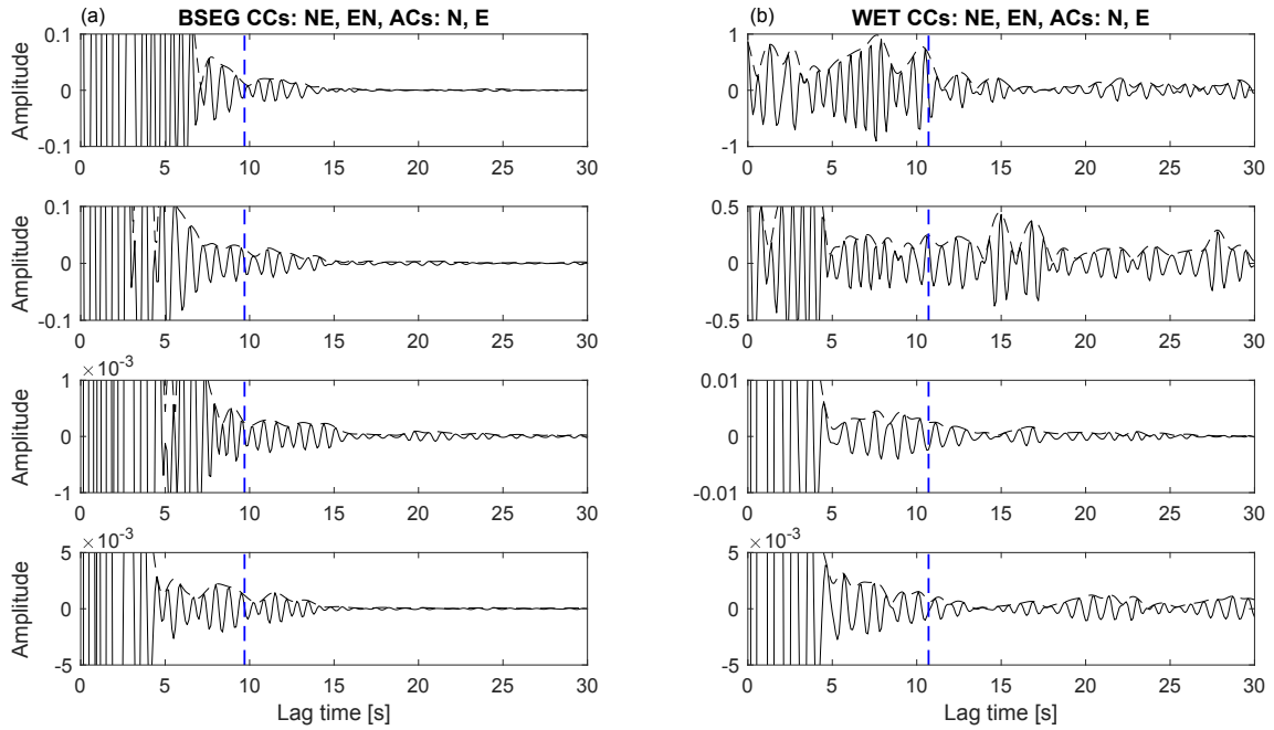
Figure 3.7: Horizontal component cross-correlations (top rows) and autocorrelations (bottom rows) for stations BSEG (left) and WET (right). Black dashed lines: envelopes. Blue lines: Expected lag time of P -wave reflectivity change (Becker & Knapmeyer-Endrun 2018).
