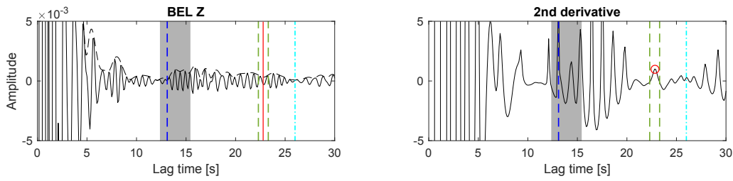
Figure 3.8: Vertical component autocorrelation with envelope (black, dashed) of station BEL (left) with corresponding second derivative. Red line/circle: Picked S -wave reflectivity change. Grey: P -wave reflectivity change target window; dark blue line: picked lag time of P -wave reflectivity change; green lines: picked lag times of S -wave reflectivity change; light blue line: picked LAB reflectivity change of P -wave
