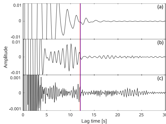
Figure 2.4: Different filtering bands applied to the autocorrelation for station GEC2. Frequency bands used: (a): 0.5-1 Hz, (b): 1-2 Hz, (c): 2-4. Red and blue lines (here overlapping) indicate calculated lag time of Moho reflected P -waves according to Grad et al. (2009) and Knapmeyer-Endrun et al. (2014).
