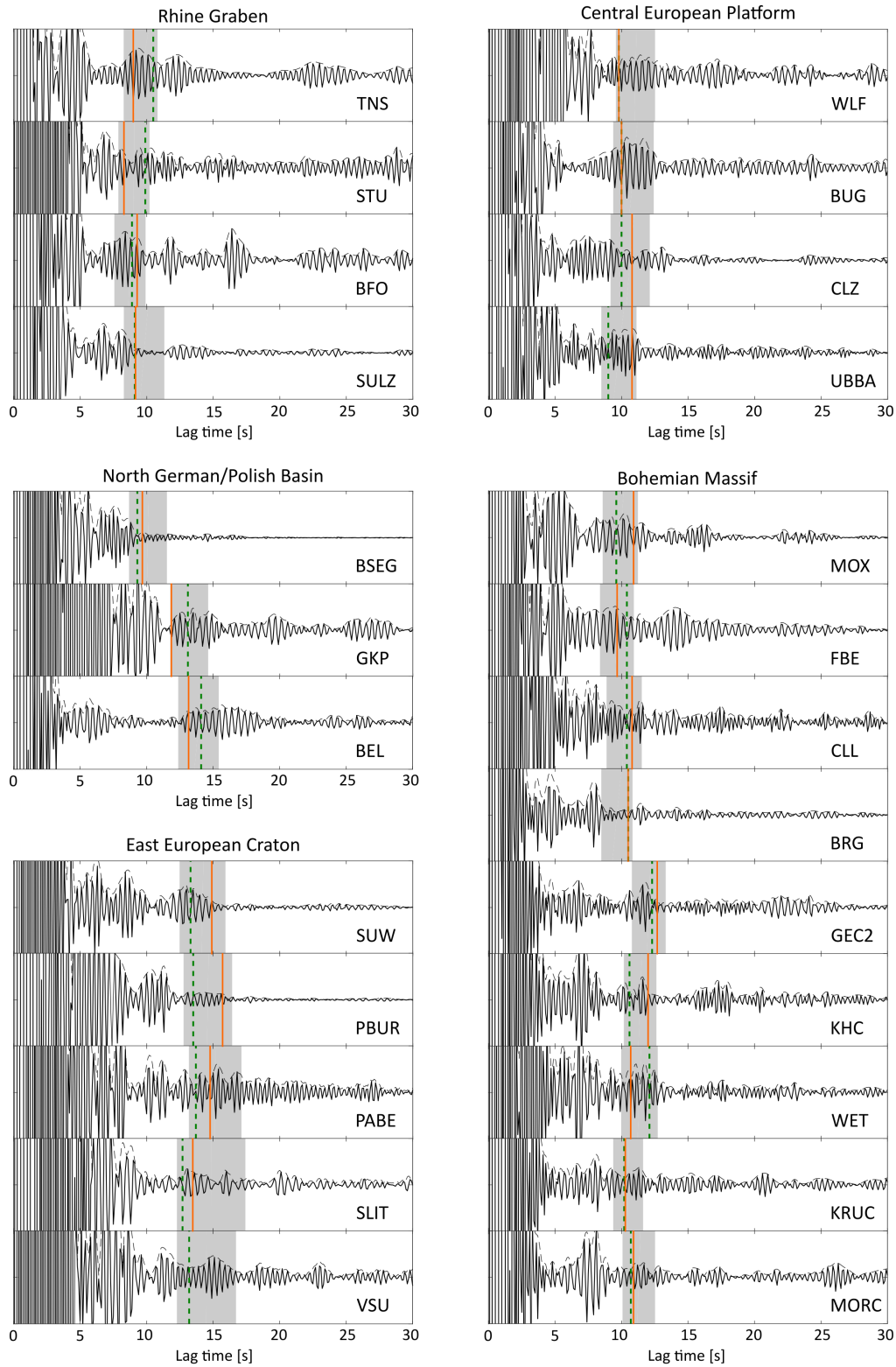
Figure A2.18: Autocorrelations filtered between 2-4 Hz in black with envelopes (dashed, black) and results of automatically picked arrival times of Moho reflections (dashed, green), along with picks made in the 1-2 Hz frequency band in orange. Grey area indicates 5 % velocity uncertainty combined with depth uncertainty provided by Grad et al. (2009).
