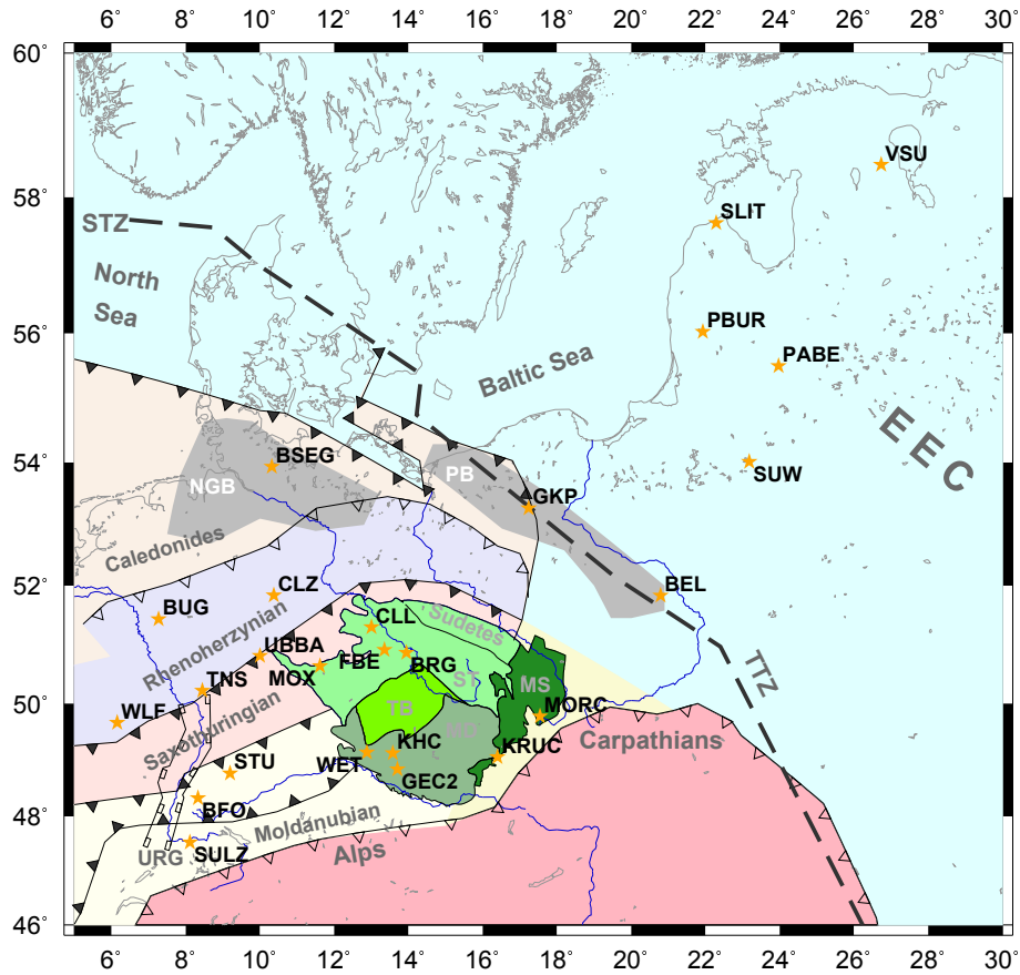
Figure 3.1: Overview of the tectonic setting of the study area (modified after Knapmeyer-Endrun et al. (2014)). Orange stars indicate the broad-band stations used. Labels: EEC: East European Craton; MD: Moldanubian of Bohemian Massif; MS: Moravo-Silesian of Bohemian Massif; NGB: North German Basin; PB: Polish Basin; ST: Saxothuringian of Bohemian Massif; STZ: Sorgenfrei-Tornquist Zone; TB: Tepla-Barrandian of Bohemian Massif; TTZ: Teisseyre-Tornquist-Zone; URG: Upper Rhine Graben
