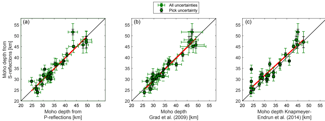
Figure 3.10: Comparison of Moho depths determined here with results from Becker & Knapmeyer-Endrun (2018) (a), Grad et al. (2009) (b) and Knapmeyer-Endrun et al. (2014) (c). Black symbols indicate uncertainty originating from the two picks of the horizontal component correlations. Green symbols indicate uncertainty resulting from uncertainty in the velocity used for converting lag time to depth, as well as uncertainty provided by the studies. The black lines have a slope of 1, whereas the red lines indicate the lines of best fit.
